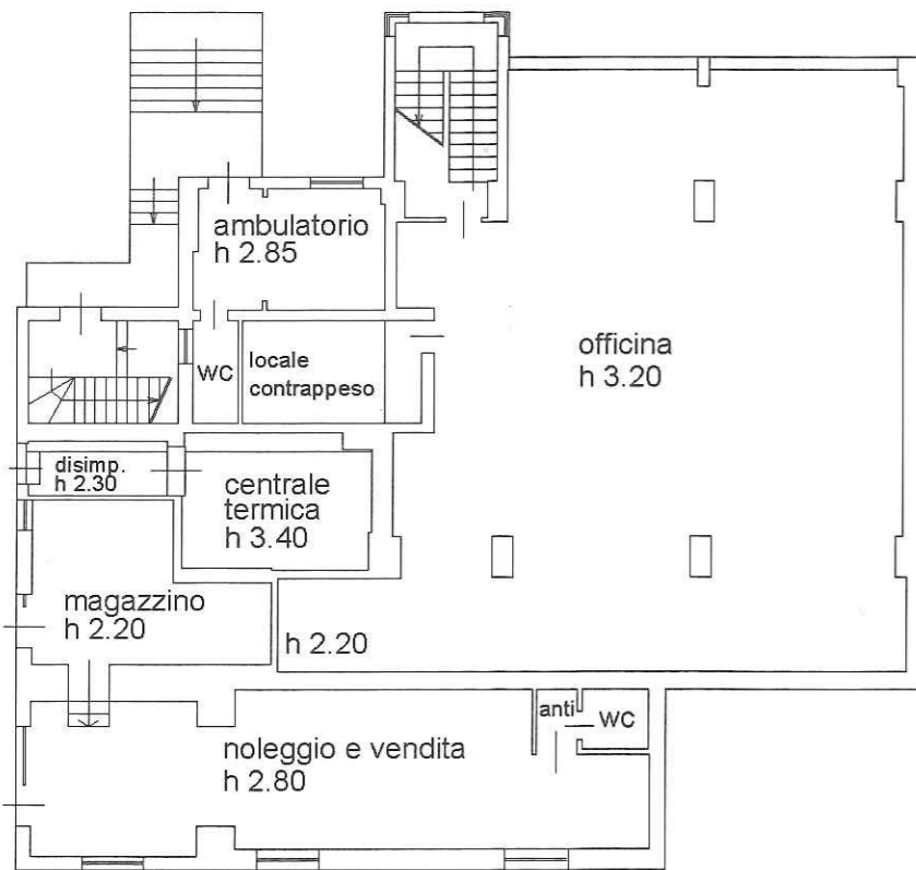
PIANO TERRA
